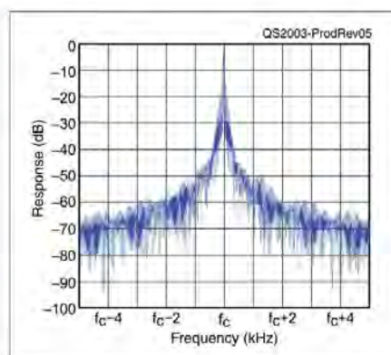
Figure 5 — Spectral display of the Xiegu G90 transmitter during keying. Equivalent keying speed is 60 WPM using external keying. Spectrum analyzer resolution bandwidth is 10 Hz, and the sweep time is 30 seconds. The transmitter was being operated at 19 W PEP output on the 14 MHz band, and this plot shows the transmitter output ±5 kHz from the carrier. The reference level is 0 dBc, and the vertical scale is in dB.
