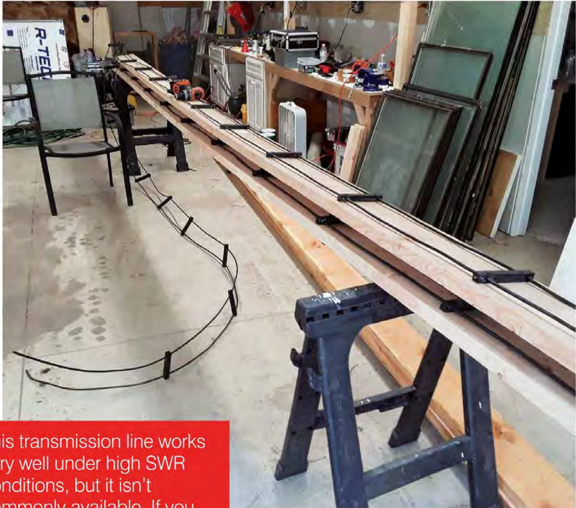
Open-wire line with spacers every 2 feet, shown under construction.
