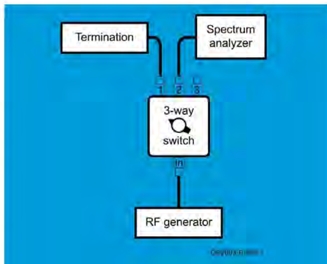
Figure 1 — A diagram of the author's isolation test setup, which consists of a Keysight N5173B RF generator, a Keysight N901A spectrum analyzer, a 50 Ω termination, and the MFJ-2703 three-way switch.
