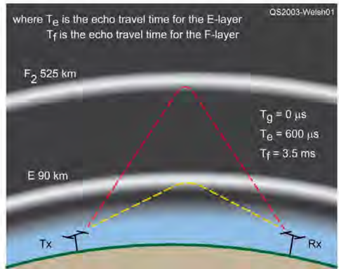
Figure 1 — A low-power ionosonde simultaneously measures seven observable parameters of reflected signals received from the ionosphere to estimate the height of the ionosphere. Here, T_e is the echo travel time for the E-layer, and T_f is the echo travel time for the F-layer.
