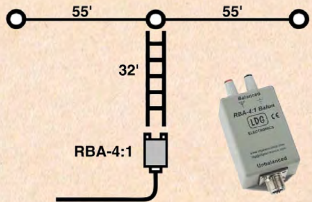
G5RV DIPOLE
