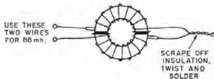
Fig. 3 — This drawing shows the method for connecting the toroid windings to obtain the required 88-mH inductance.
