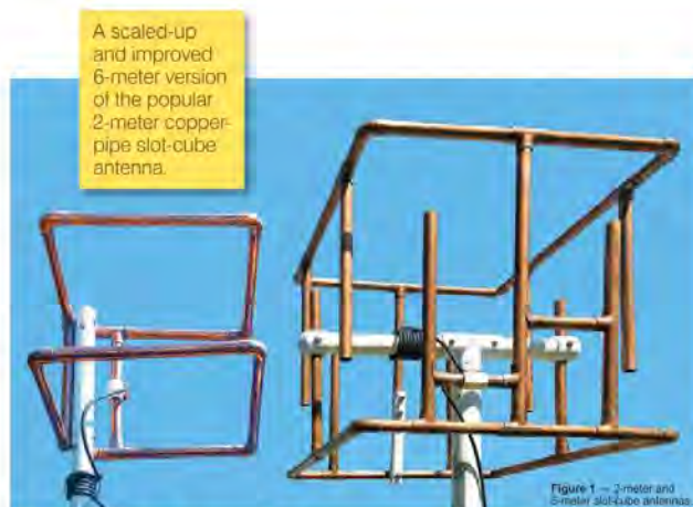
Figure 1 — 2-meter and 6-meter slot-cube antennas
